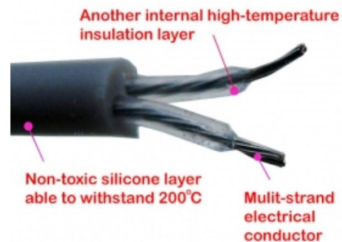
Temperature Probe Cable Structure
